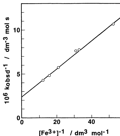
Fig. 3. Plot of k_{\text{obsd}}^{-1} vs. [\text{Fe}^{3+}]^{-1} for the decay of \text{RAn}^{\bullet+} ( \text{R} = \text{PhCH}_2 ) formed in the electron-transfer oxidation of \text{RAn} ( 6.25 \times 10^{-4} \text{ mol dm}^{-3} ) by \text{Fe}(\text{ClO}_4)_3 in \text{MeCN} at 298 K.
